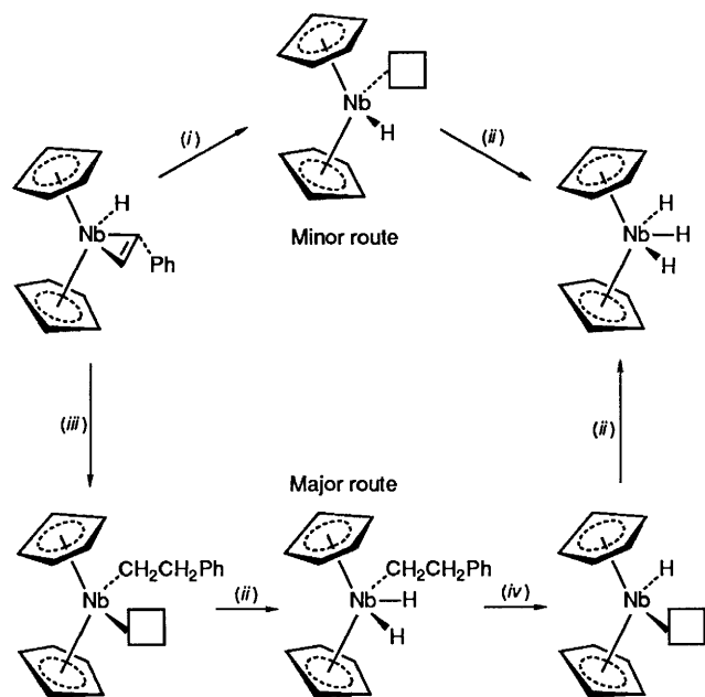
Scheme 2 Mechanism proposed for the reaction of endo -[Nb( \eta\text{-C}_5\text{H}_5 ) 2 ( \eta\text{-H}_2\text{C=CHPh} )H] with hydrogen. (i) Dissociation of styrene; (ii) oxidative addition of H 2 ; (iii) olefin insertion into Nb–H bond; (iv) reductive elimination of ethylbenzene
